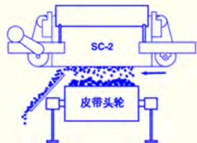
Automatic Cleaning Position SC-2
