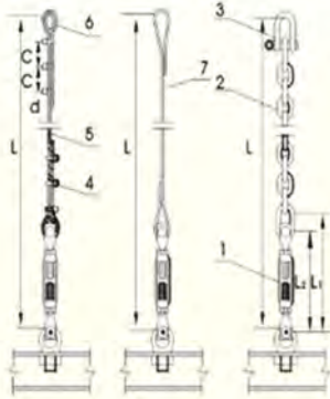
Wirerope Steel tie rode Sling
